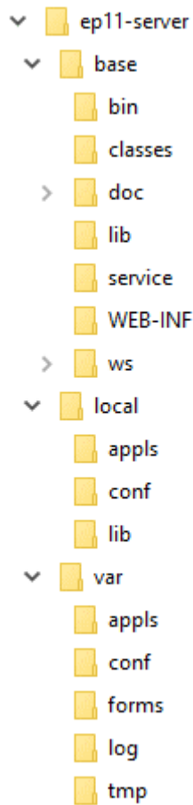
Figure 1: Directory structure
