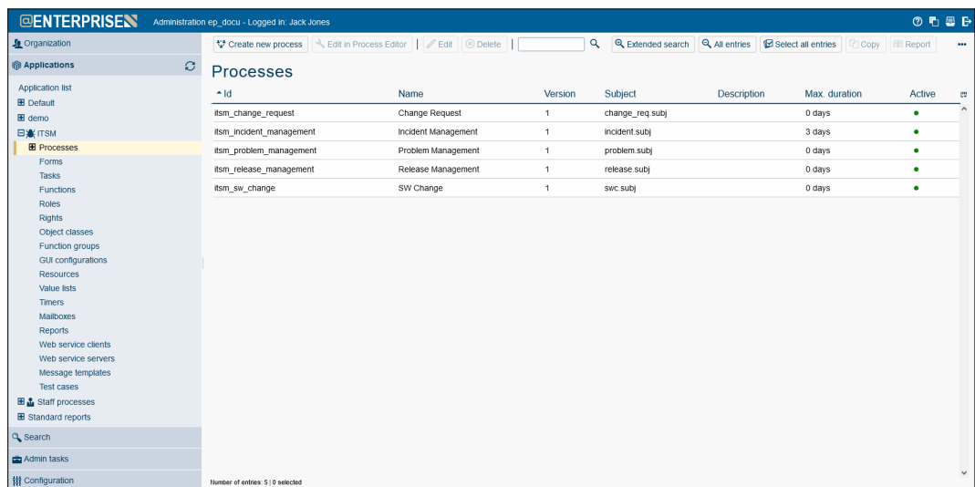
Figure 2.1: System administration
