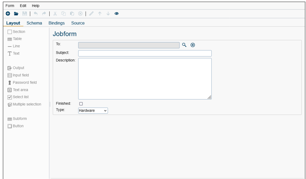
Figure 6.6: Form Editor
