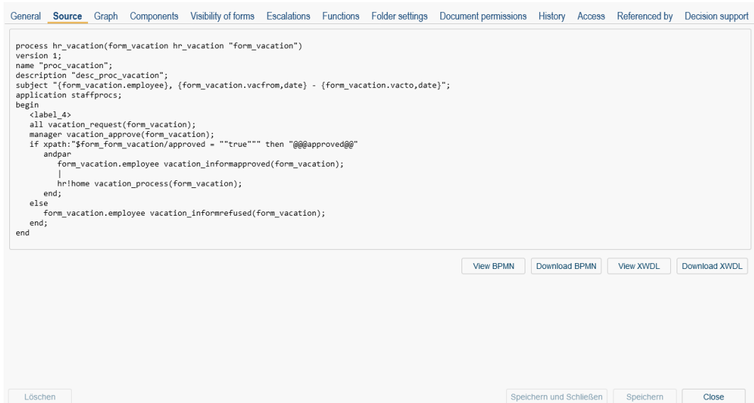
Figure 7.12: WDL source
