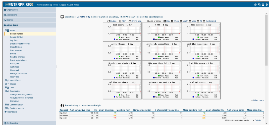
Figure 9.1: Server Monitor
