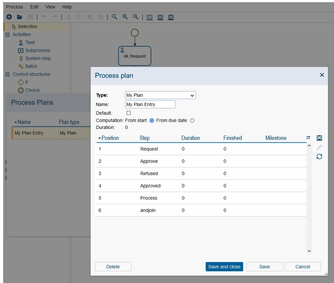
Figure 7.15: Process plans
