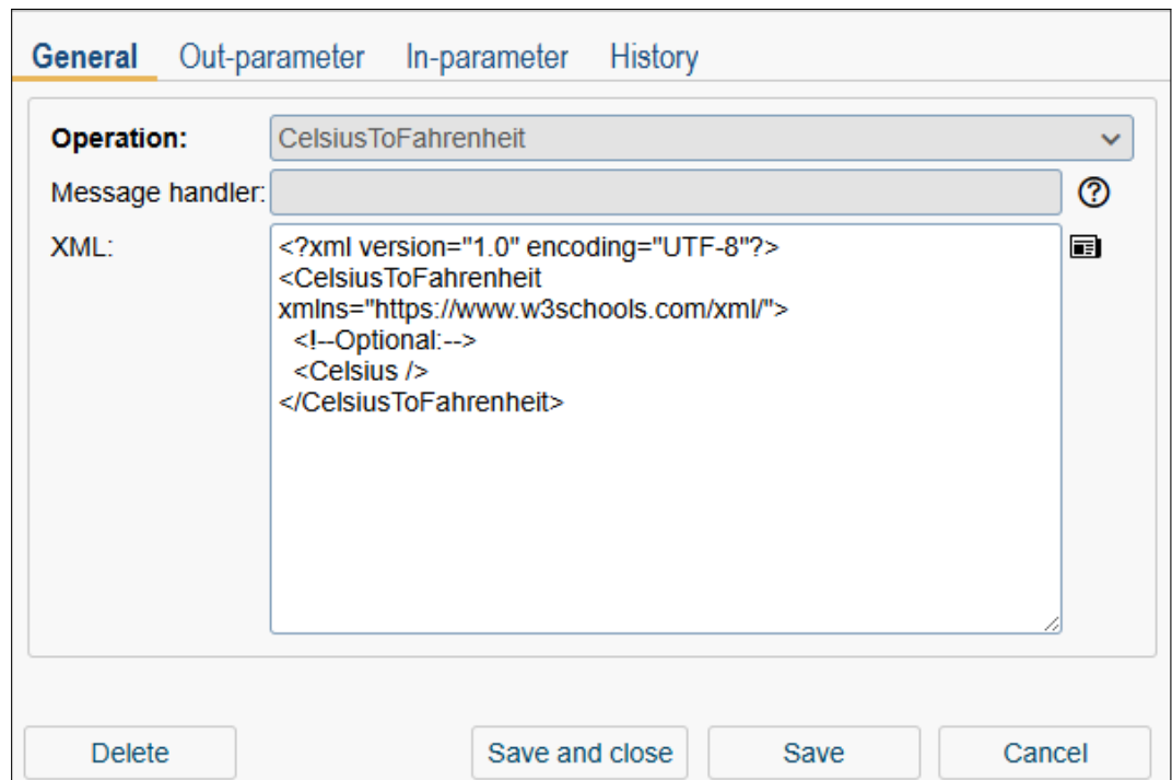
Figure 6.45: The Operation-Object
