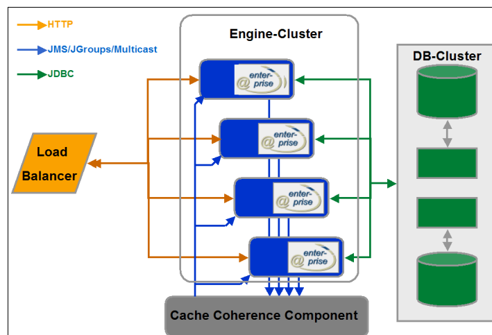
Figure 5.1: Cluster Architecture
